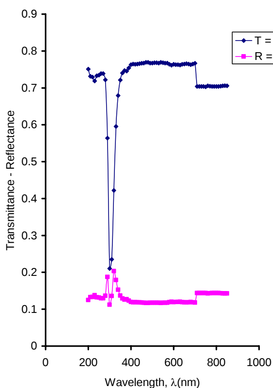
Figure 2: Transmittance-Reflectance Spectra of PbHgS Film Prepared at 300K.
