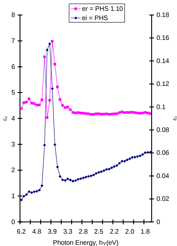
Figure 4: Plots of Real Dielectric Constant ( \epsilon_r ) and Imaginary Dielectric Constant ( \epsilon_i ) against Photon Energy for PbHgS Films.
