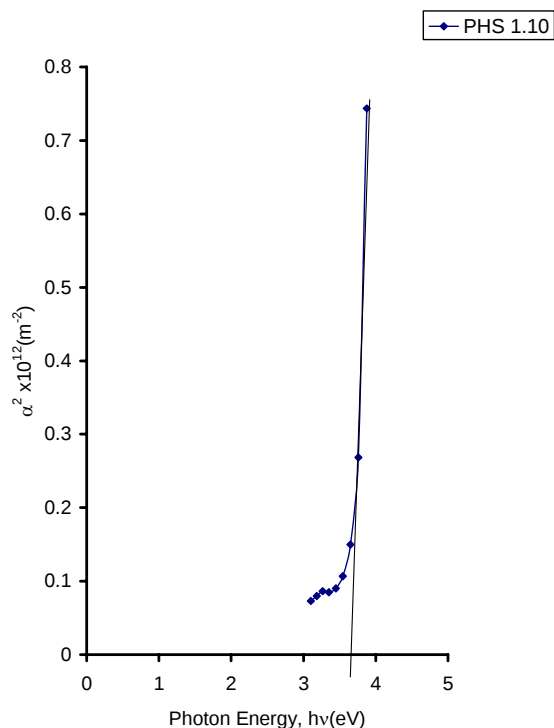
Figure 1a: The Plot of \alpha^2 Against h\nu for PbHgS Film Prepared at 300K.
