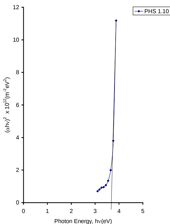
Figure 1b: The Plot of (\alpha h\nu)^2 Against Photon Energy for a PbHgS Sample.
