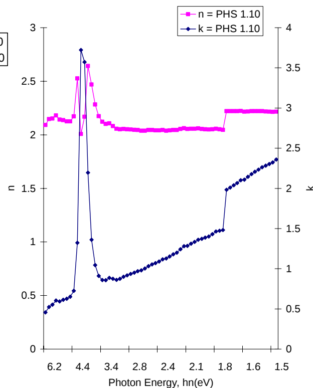
Figure 3: Plots of Refractive Index (n) and Extinction Coefficient (k) against Photon Energy for PbHgS Film Prepared at 300K.
