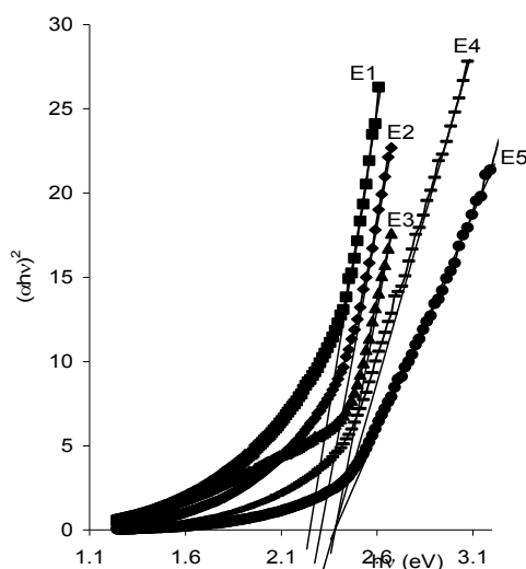
Fig. 5. Plot (\alpha h\nu)^2 vs h\nu for CdNiS thin films.
